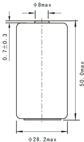
Dimensions in mm Weight: 53g
