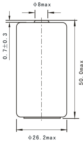
Dimensions in mm Weight: 57g
